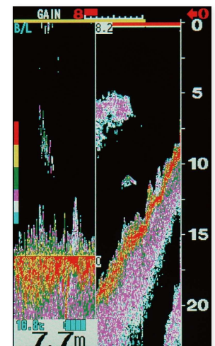
Bottom Lock + Normal
