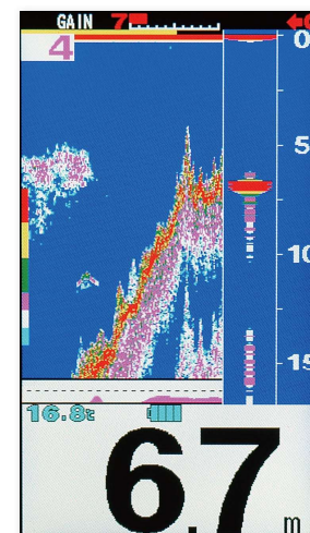
Bottom Hardness Graph
